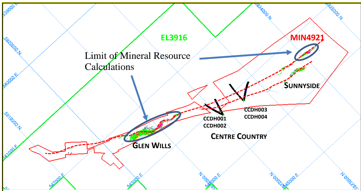
Figure 2: Resource Block Models (2012) Showing Defined Mineralisation, Previous Drilling at Centre Country Area and Projections of Potential Mineralised Extensions.
