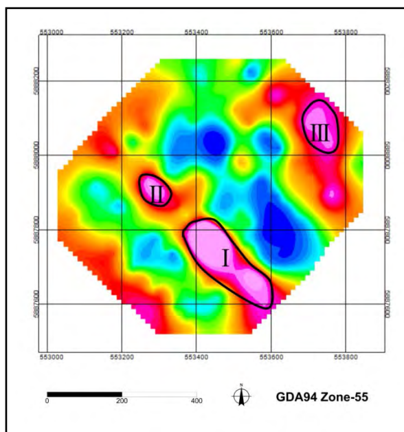
Figure 3. Inference and Interpretation Plan of Dual-Frequency IP Apparent Frequency Dispersivity Abnormity – Comstock Prospect Showing Anomalous Areas I, II & III.
